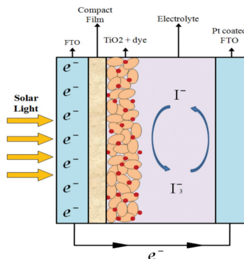
FIGURE 1. Schematic diagram of dye sensitized solar cells
